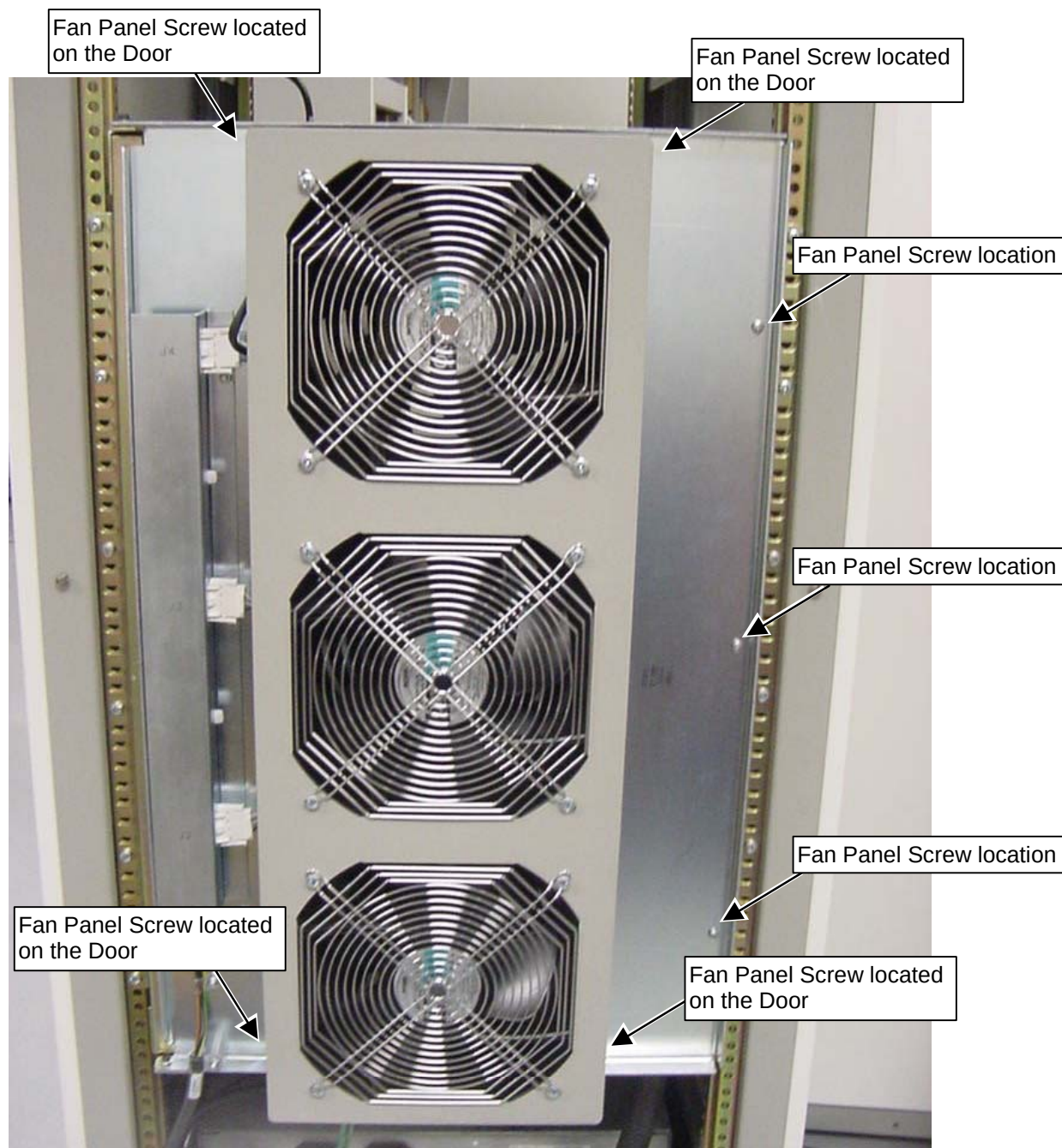
LOCATION OF SCREWS TO OPEN FAN PANEL ILLUSTRATION 1-8
